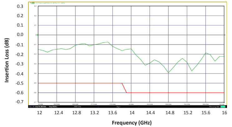
Insertion Loss (12-16 GHz)
