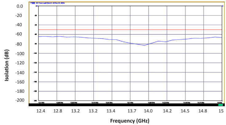
Isolation (12-15 GHz)
