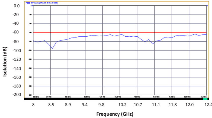
Isolation (8-12.4 GHz)
